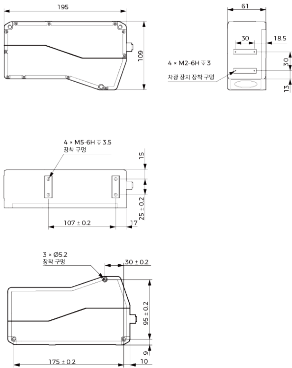
Mech-Eye LNX-8080-GL
