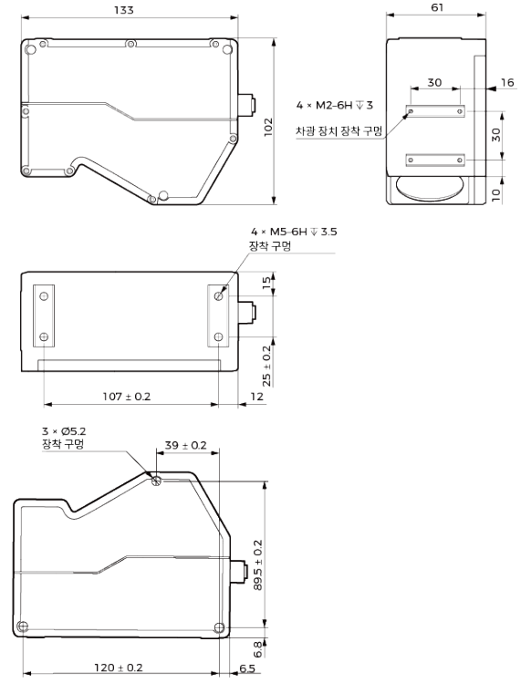
Mech-Eye LNX-8300-GL
