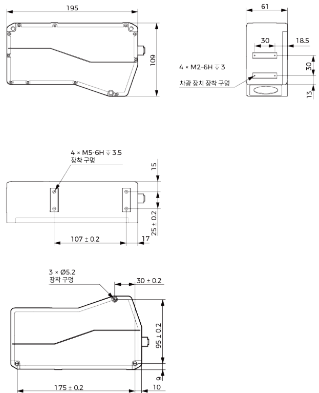
Mech-Eye LNX-8300-GL
