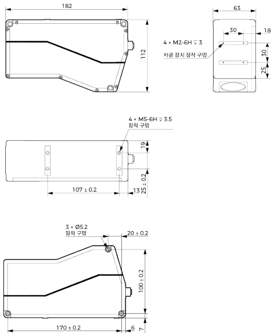
Mech-Eye LNX-7580-GL
