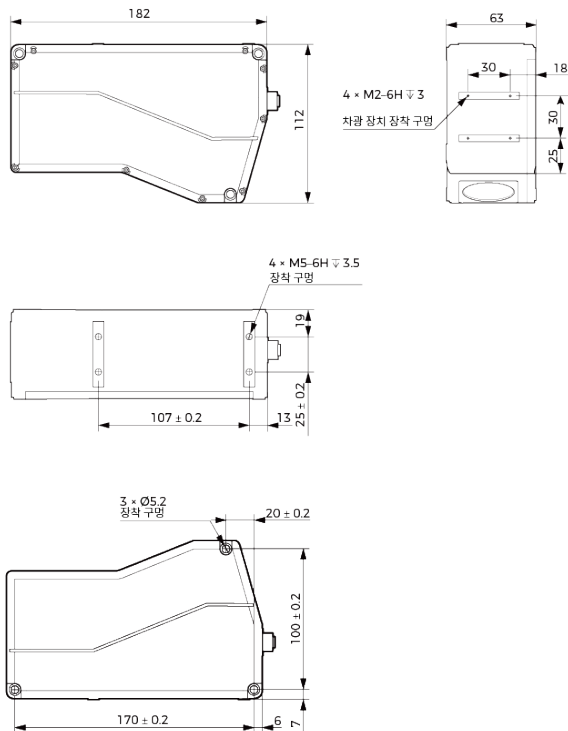
Mech-Eye LNX-8080-GL
